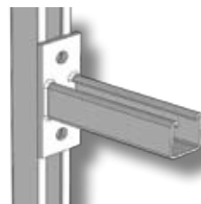
Size mm Cat. No. Size mm Cat. No. 150mm LONG ARM TC103-15 600mm LONG ARM TC103-60 300mm LONG ARM TC103-30 750mm LONG ARM TC103-75 450mm LONG ARM TC103-45
