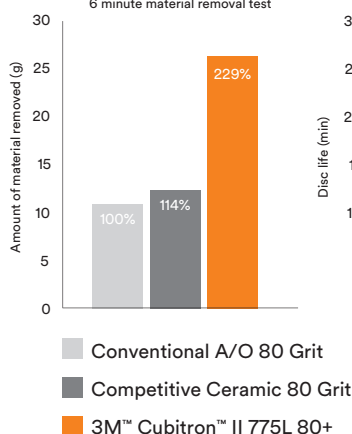
3M Precision Shaped Ceramic Grain
