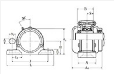
Pillow Block Unit, Set Screw, Cast Dust Cover, Closed End, UCP Type - Dimensions
