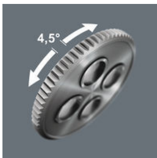
The Zyklus VDE ratchet allows a short return angle of only 4.5 ° thanks to its 80 teeth.
