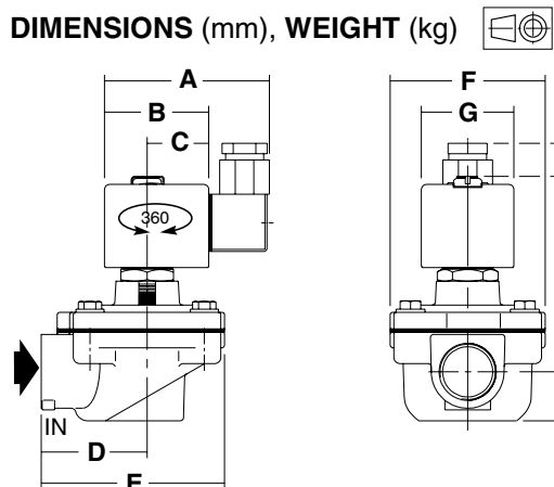
Fig. 1 threaded type
