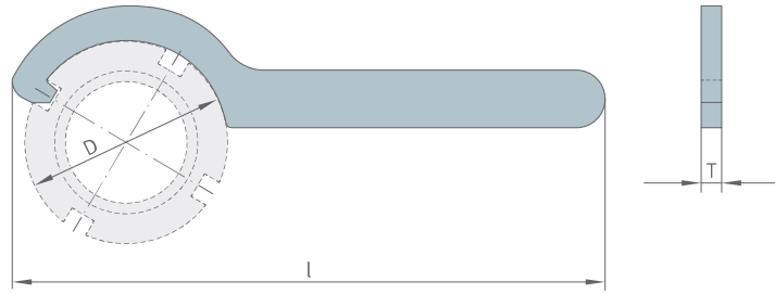
9 LOCKNUT-HOOK dimensions
