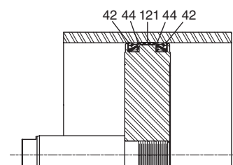
Lipseal Piston with Wear Ring 2A Series Bores 8, 10, 12 & 14
