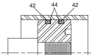
Lipseal Piston (All Series)
