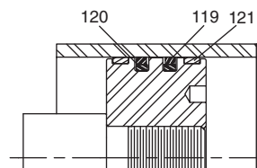
Hi-Load Piston (All Series except 2A & 3L)
