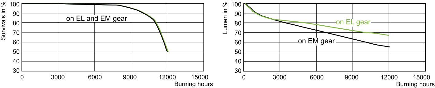
CDM-T 70W Life Expectancy /830
