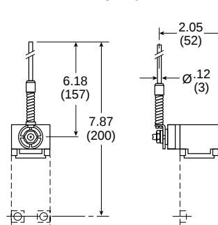
ZCKY91
