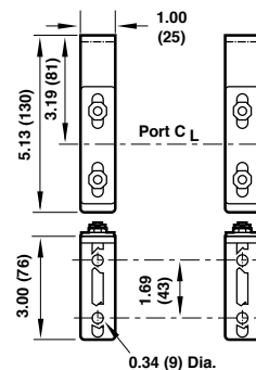
F17, F46 Bracket (6212-50, 6212-51)
