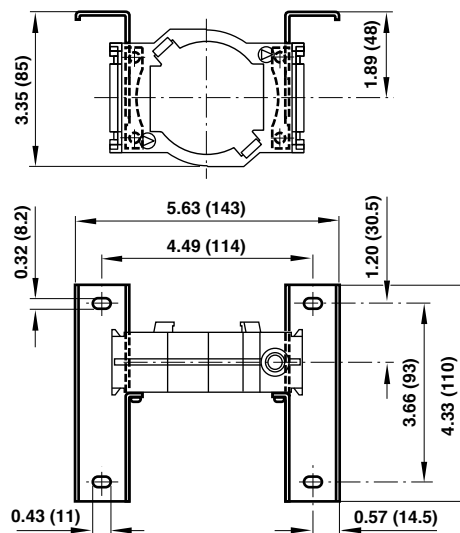
F64 Bracket (74504-50)
