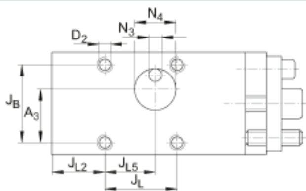
View X
