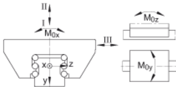
Load directions
