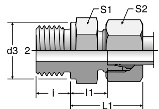
Cutting face DIN 3852, form B, G (BSPP) thread
