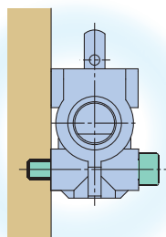
Side mounting
