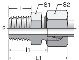
R (BSPT) thread
