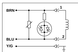
Circuit
