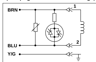
Circuit
