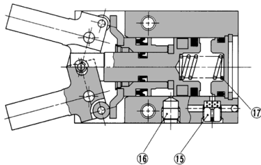
Single acting
