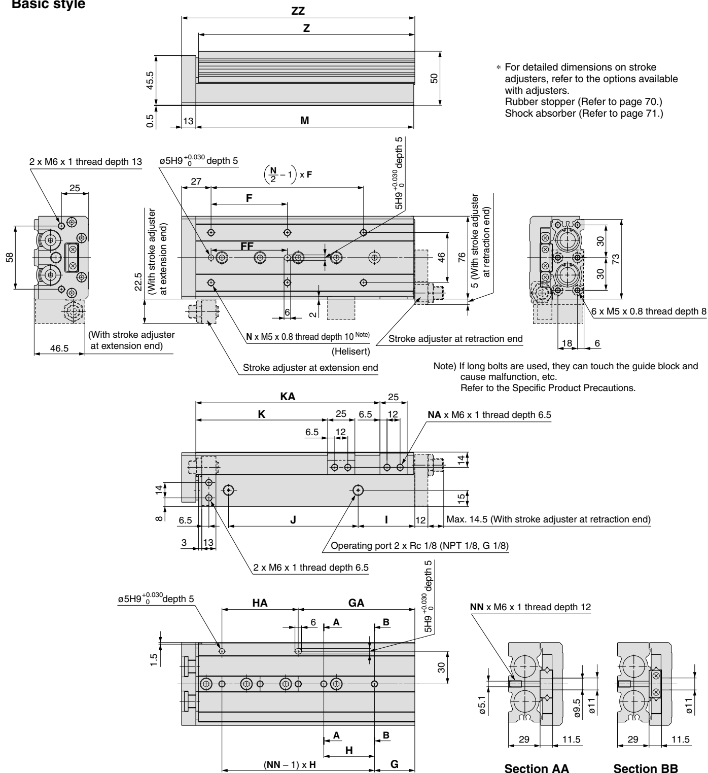
Section AA
