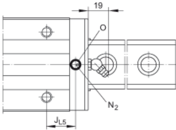
Lubrication connector in top face
