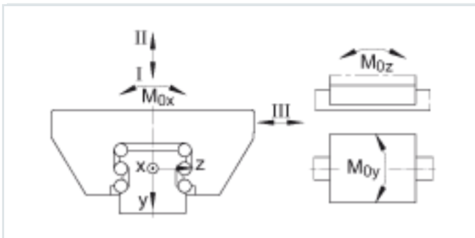
Load directions
