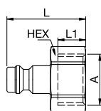
Female Thread
