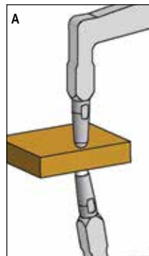
Ball Ø 1.5 and 3mm for wall thickness
