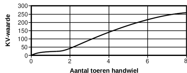
BSAT - DN200
