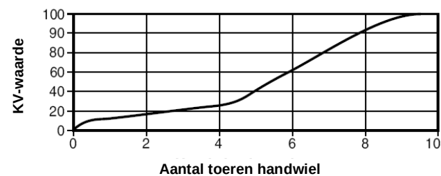
BSAT - DN125
