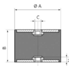
Type C 0 Studs
