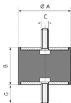
Type A 2 Studs
