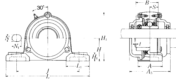
Cast dust cover type Open end C-UCP...D1 Closed end CM-UCP...D1
