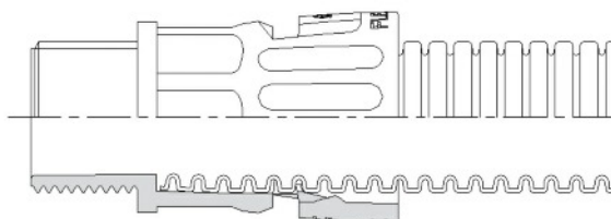
FPAL Conduit with FLK fitting
