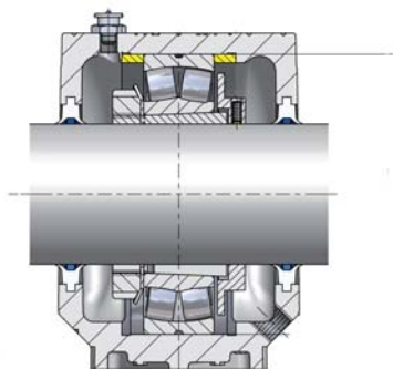
Double lip seal SC..DS + Regulation disc RDC
