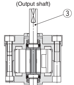
Double shaft type
