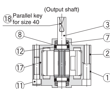
Single shaft type
