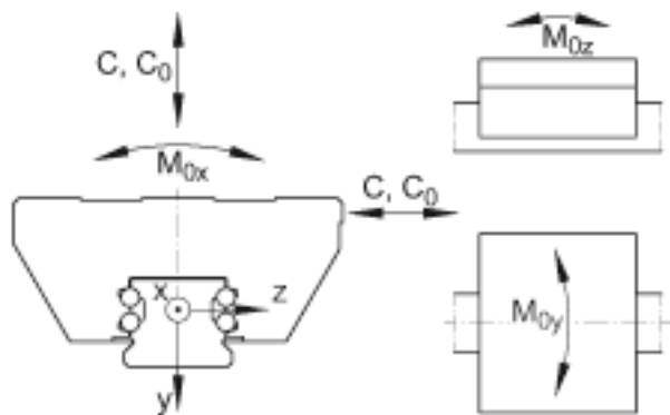
Load directions
