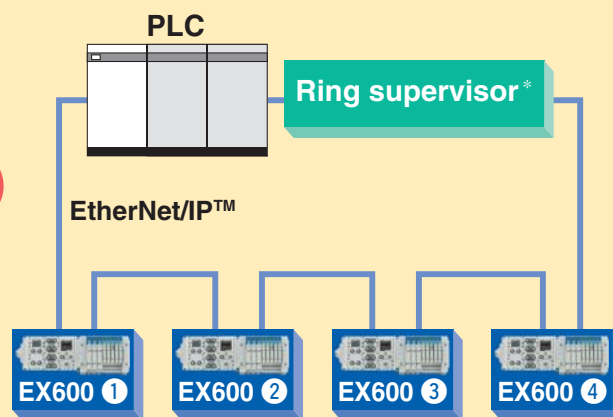
Device level ring (DLR) type
