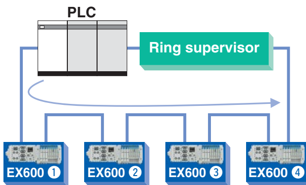
Normal flow of data
