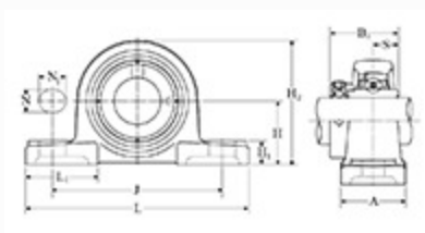
Pillow Block Unit, Cast Housing, Eccentric Locking Collar, UELP/UELPL Type - Dimensions
