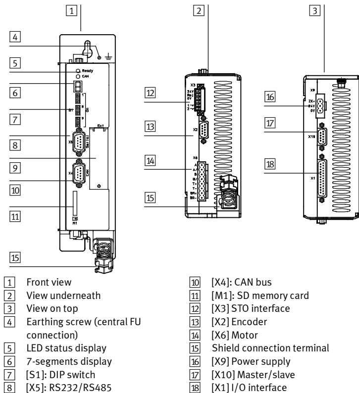
Fig. 1 Motor controller CMMS-ST-...-G2
