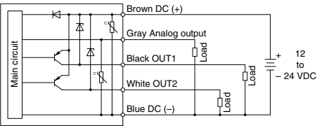
PSE304(T) PNP (2 outputs) + Analog current output
