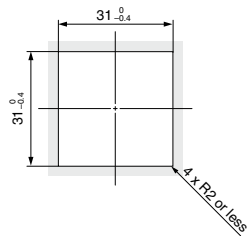
Mount of single unit
