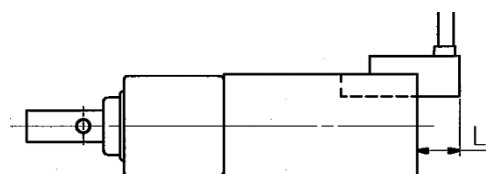
When using auto switch D-M9□V
