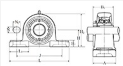
Pillow Block Unit, Adapter, Cast Housing, UKP Type - Dimensions
