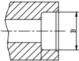
Socket weld bore
