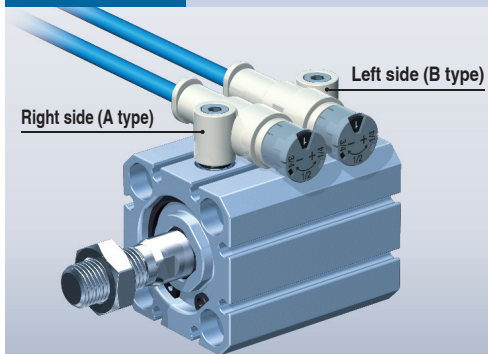
Installation example Reducing protrusion of JAS-S body over rod end and head end
